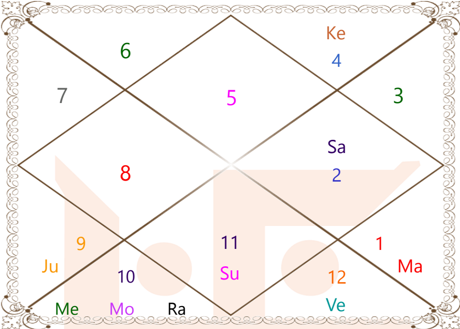
Lagna Chart
