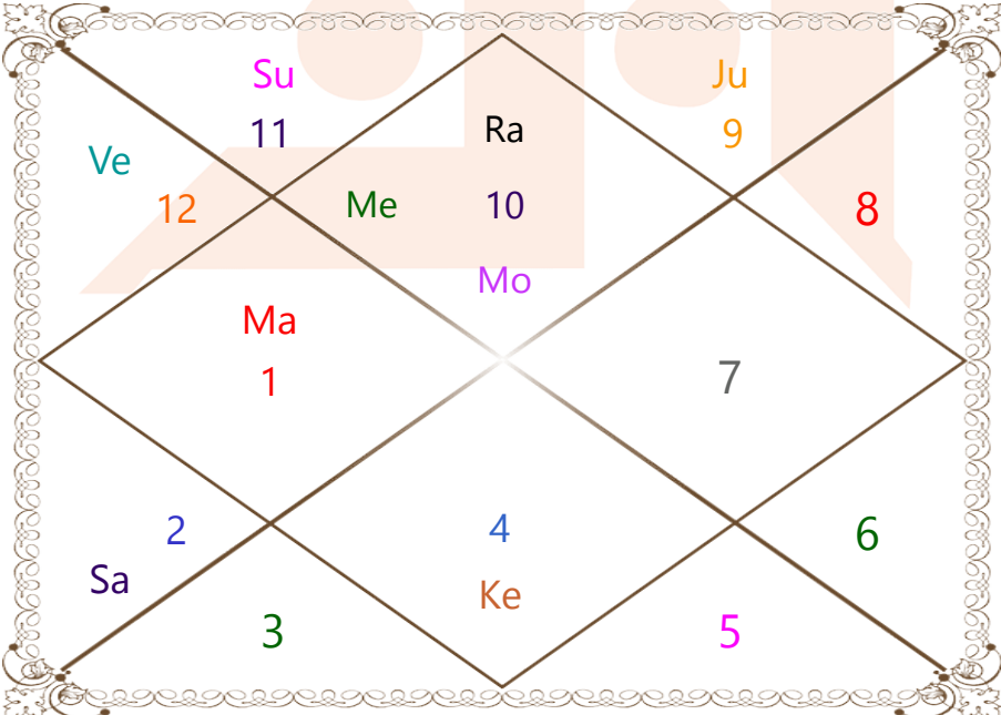
Moon Chart
