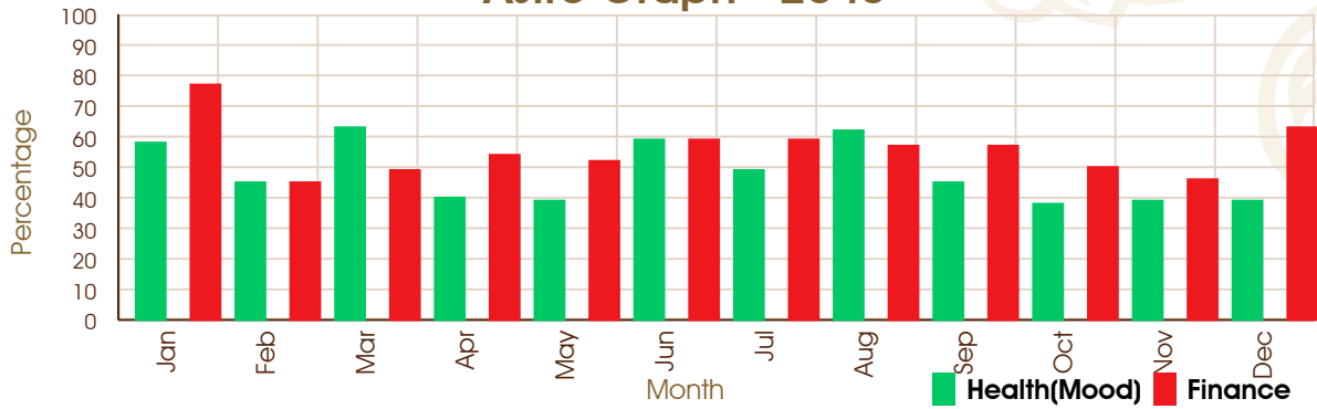
Astro Graph - 2041
