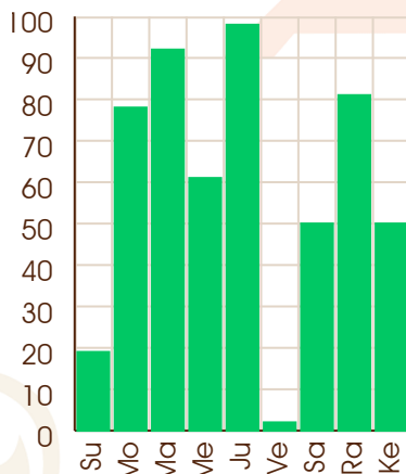
Rahu - 05/08/2045
