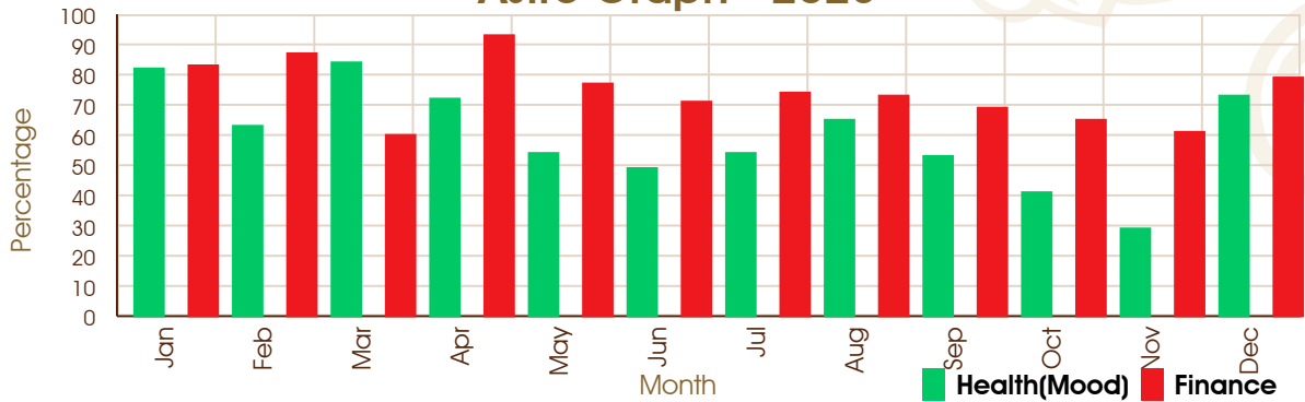
Astro Graph - 2029
