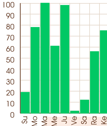
Ketu - 05/08/1984
