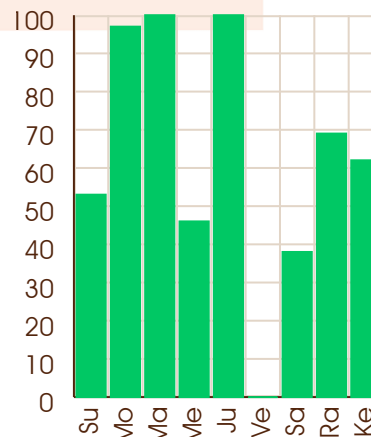
Jupiter - 05/08/2061
