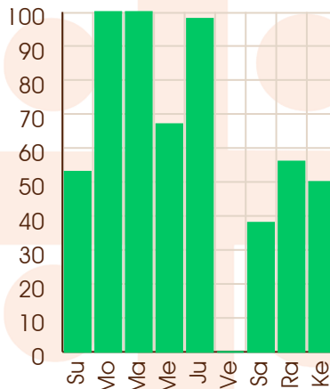
Moon - 05/08/2020
