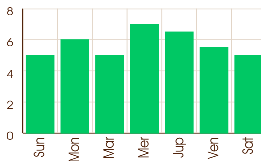
Minimum Shadbala
