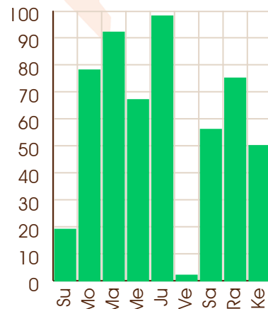
Saturn - 05/08/2080
