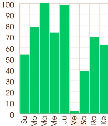
Mercury - 05/08/1977
