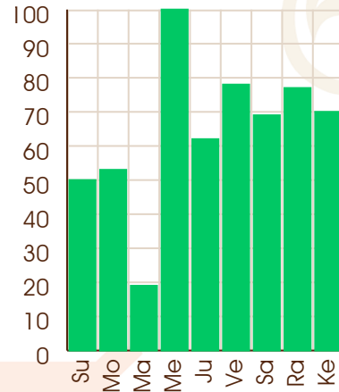
Venus - 09/07/2023
