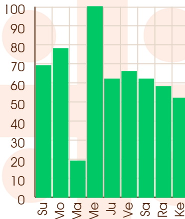
Moon - 09/07/2039
