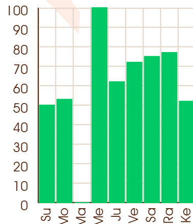
Saturn - 09/07/2099
