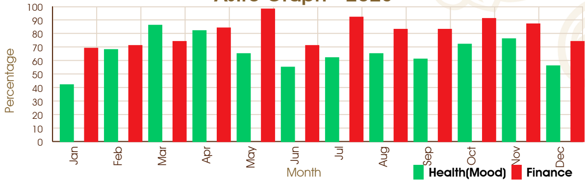
Astro Graph - 2024
