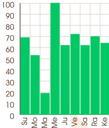
Mercury - 08/07/1996
