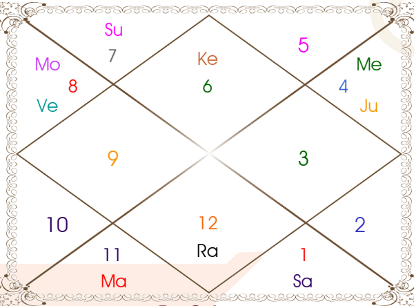
Dreshkana Chart
