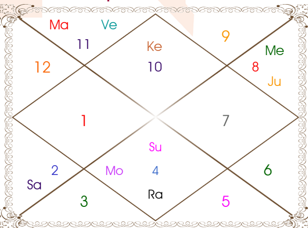
Saptamamsa Chart
