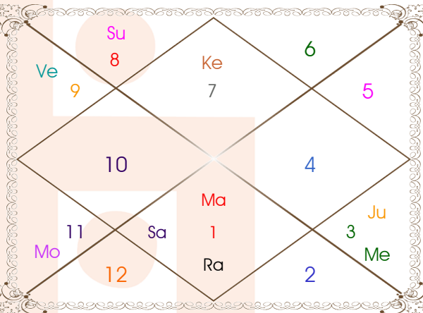
Chaturthamsa Chart
