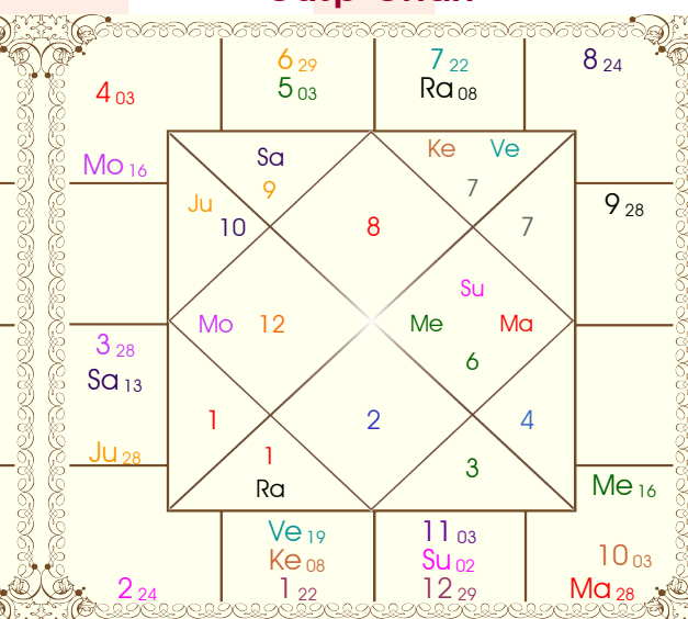
Cusp Chart
