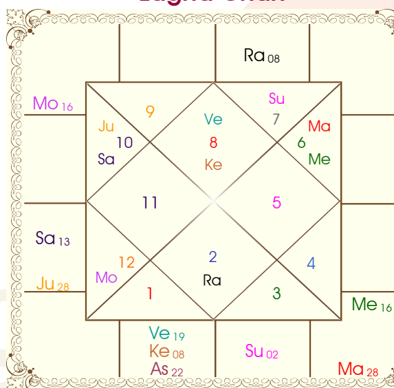
Lagna Chart
