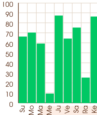
Mercury - 26/07/2048
