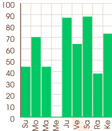
Saturn - 27/07/2031
