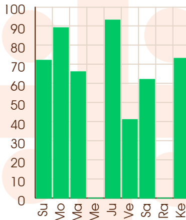
Sun - 27/07/2081
