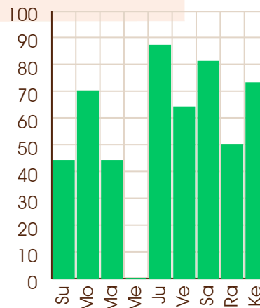
Rahu - 27/07/2116
