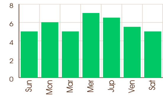
Minimum Shadbala
