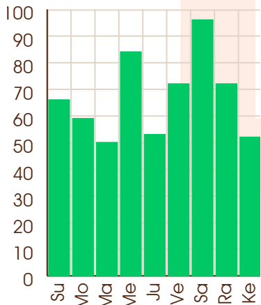
Sun - 27/09/2031
