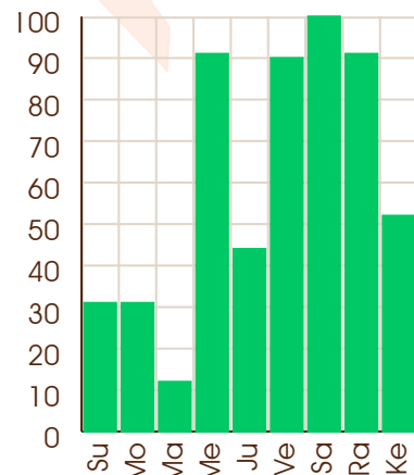
Saturn - 28/09/2101
