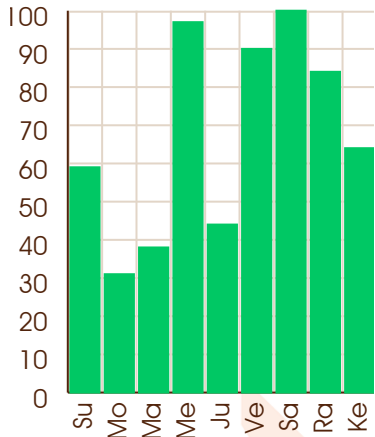
Mercury - 27/09/1998
