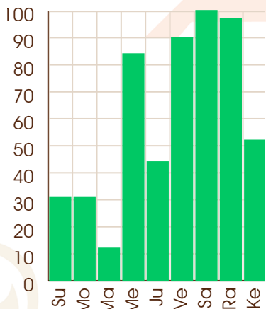
Rahu - 27/09/2066
