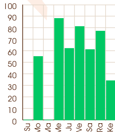
Rahu - 20/02/2107
