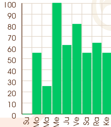
Mercury - 19/02/2039
