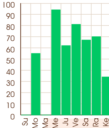
Saturn - 19/02/2022
