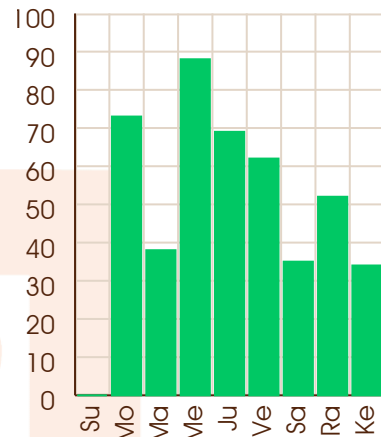
Sun - 19/02/2072
