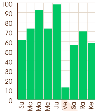
Mercury - 02/04/1994
