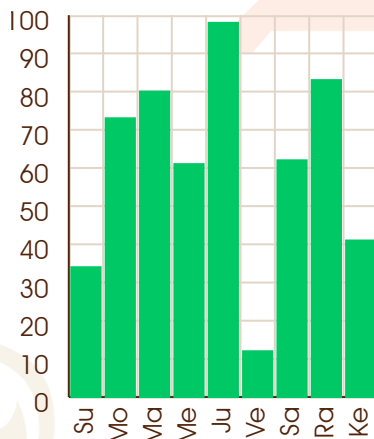
Rahu - 02/04/2062
