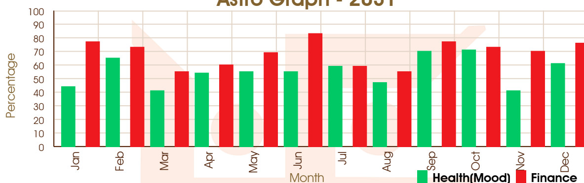
Astro Graph - 2032
