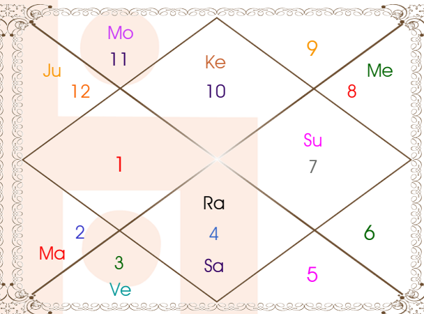
Dasamamsa Chart
