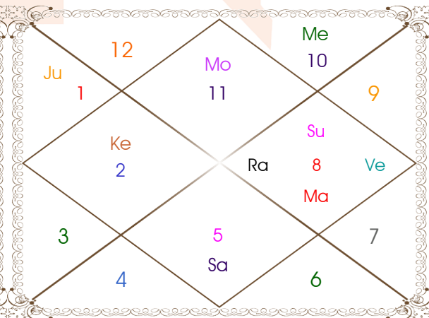
Dwadasamsa Chart
