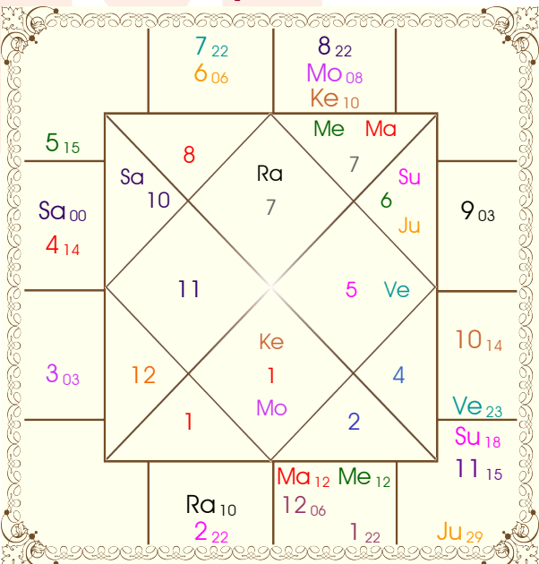
Cusp Chart
