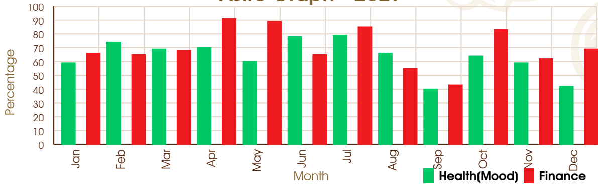
Astro Graph - 2030
