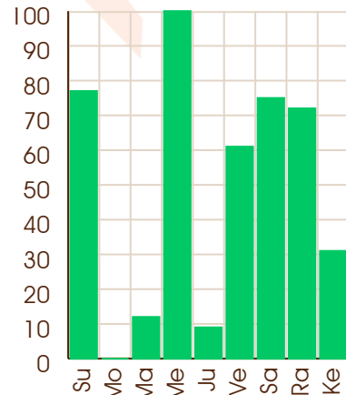
Mercury - 02/02/2102
