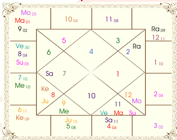
Cusp Chart
