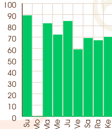
Mercury - 06/07/2032
