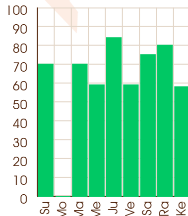
Rahu - 07/07/2100
