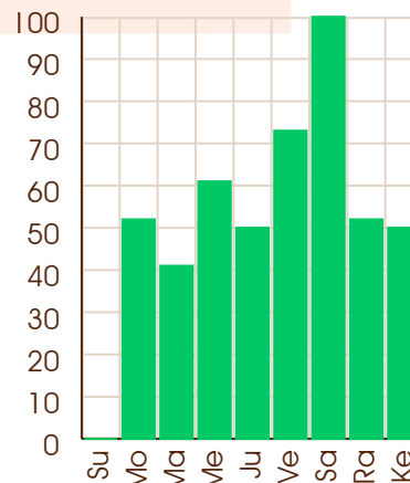
Rahu - 21/02/2078
