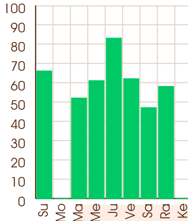
Rahu - 07/11/1989
