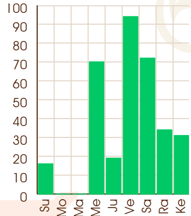
Saturn - 31/01/2039
