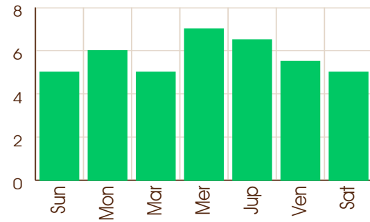
Minimum Shadbala
