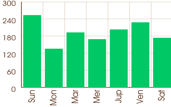
Kala Bala
