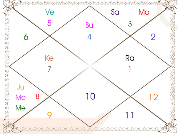
Saptavimsamsa Chart
