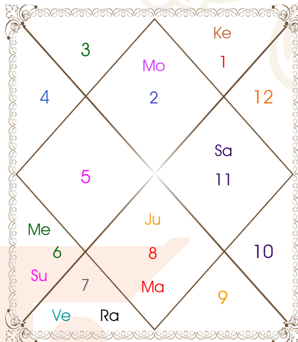
Moon Chart
