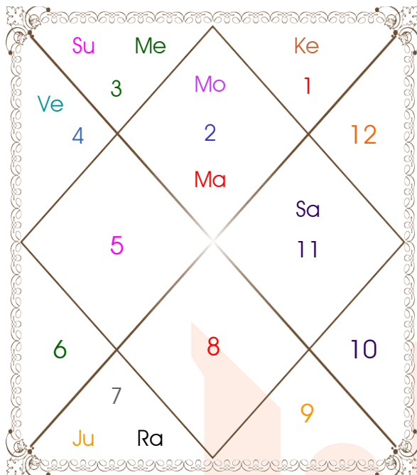
Moon Chart
