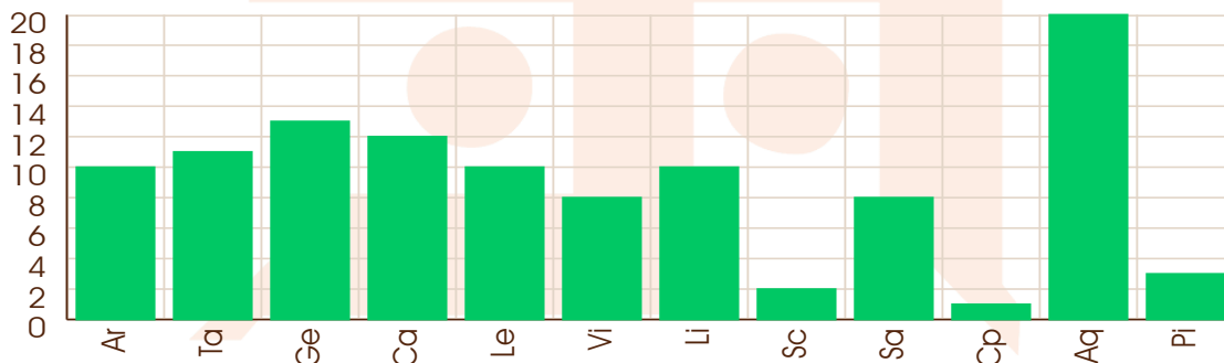
Ashtakvarga After Ekadhipatya Reduction
