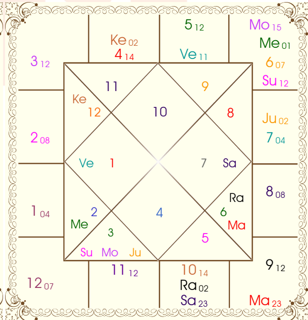
Cusp Chart
