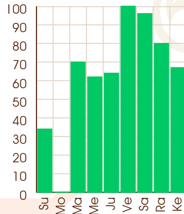
Venus - 26/07/1993
