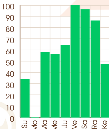
Rahu - 26/07/2034
