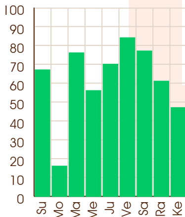
Sun - 26/07/1999
