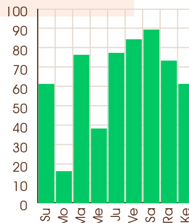
Jupiter - 26/07/2050
