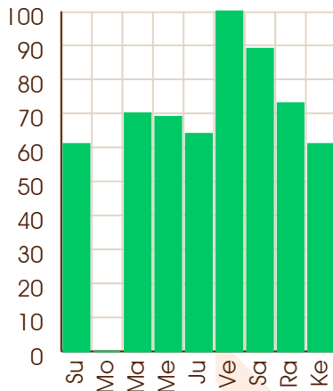
Mercury - 26/07/1966
