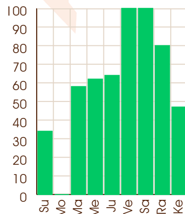
Saturn - 26/07/2069
